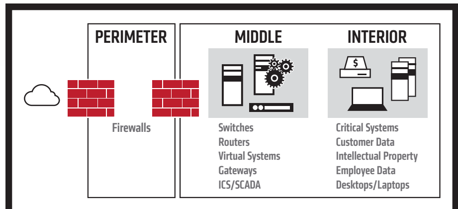
◆ FIG. 2 Tripwire Security Configuration Management—Tripwire CCM Express and Tripwire Enterprise—covers the entire enterprise.
